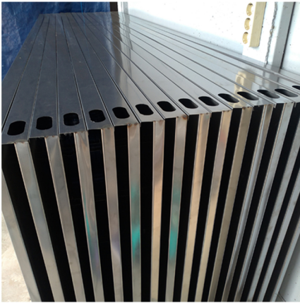
PLATE SETTLERS
